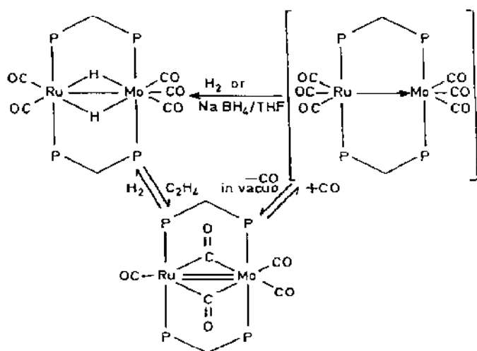
Fig. 16. Dppm bridged Mo-Ru complexes exhibiting a facile heterobimetallic activation of H_2 .
